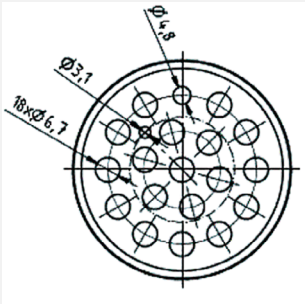
Insert Part Number: 410-3033-H
