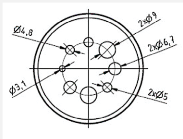
Insert Part Number: 410-3037-H
