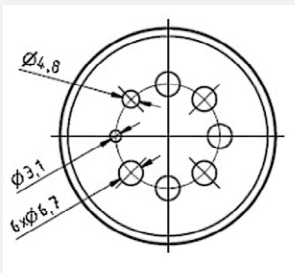
Insert Part Number: 410-3036-H
